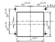
2104 Panel Cutout
